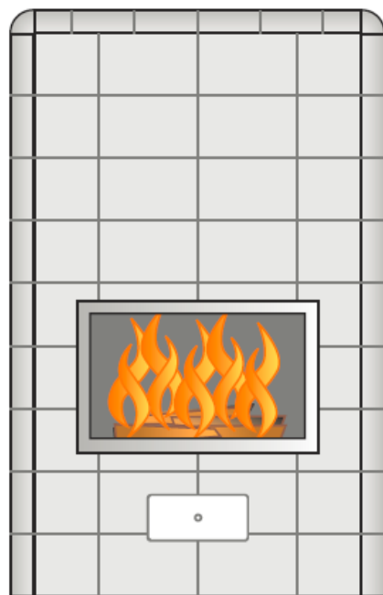
Standardmodel
